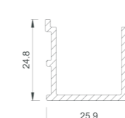
COR-4702 One rail frame with fixed isolation
