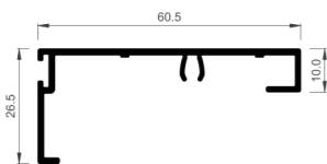
COR-4743 Fixed sash frame cover
