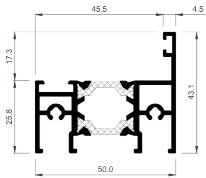
COR-4725 Central sash
