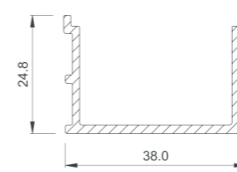
COR-4701 Two rail frame isolation
